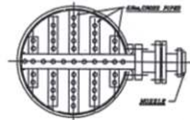
PTFE DISTRIBUTOR & DIP TUBE DETAILS
